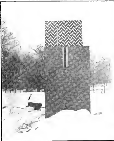
Fig. 1 —Test Object and Observer's Station at Mayfield Country Club, where early experimental work on Field-glasses took place
